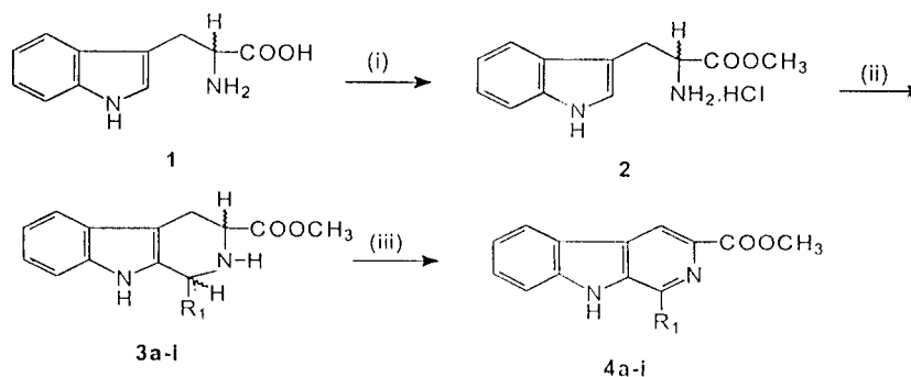
Scheme 1. Reagents: (i) MeOH, \text{SOCl}_2 ; (ii) \text{R}_1\text{CHO} , MeOH, 10% aq \text{Na}_2\text{CO}_3 ; sulphur, xylene reflux.
