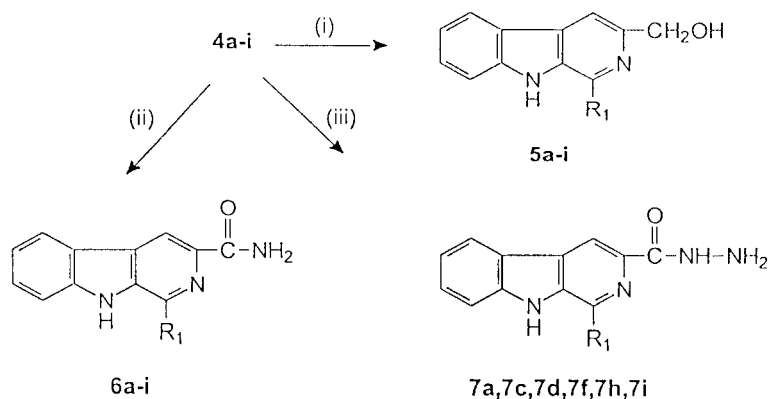
Scheme 2. Reagents: (i) \text{LiAlH}_4 dry THF, reflux, 10% aq \text{NaOH} ; (ii) aq ammonia, MeOH, 80^\circ\text{C} ; (iii) hydrazine hydrate, EtOH, reflux.
